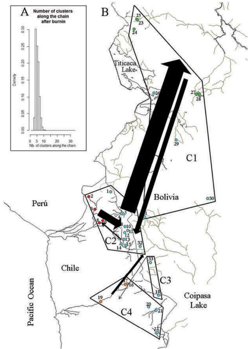
Figure 5. (a) Probability density for the number of populations simulated and obtained with Geneland. (b) Spatial distribution of each cluster (C1 to C4), defined by Geneland at K = 4. Cluster codes and basins included in each cluster are detailed in Table 1. Arrows show the Migrate gene flows between basins (see details in Table 4).
