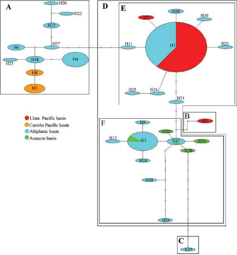
Figure 4. Haplotype network inferred using cyt-b gene sequences by statistical parsimony (TCS), for the Telmatobius marmoratus species complex. Color codes correspond to basin systems as shown in Figure 1. White circles indicate mutational steps, for details of haplotype codes see Table 1.
