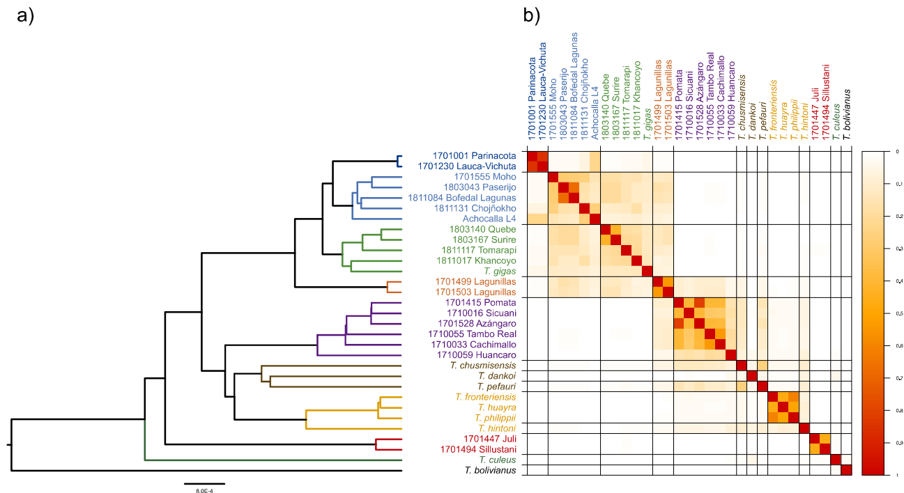
Fig. 4. a) Minimal Cluster Tree based on two mitochondrial (16S and Cytb) and two nuclear (RAG1 and BFIB) loci with b) similarity matrix obtained in Species Delimitation Analyser. The color scale shows the posterior probability of two pairs of individuals to belonging to the same cluster (species). Red is for 1.0 posterior probability and white for 0.0. The colors of the tips correspond to the phylogeny groups in Fig. 2. (For interpretation of the references to color in this figure legend, the reader is referred to the web version of this article.)
