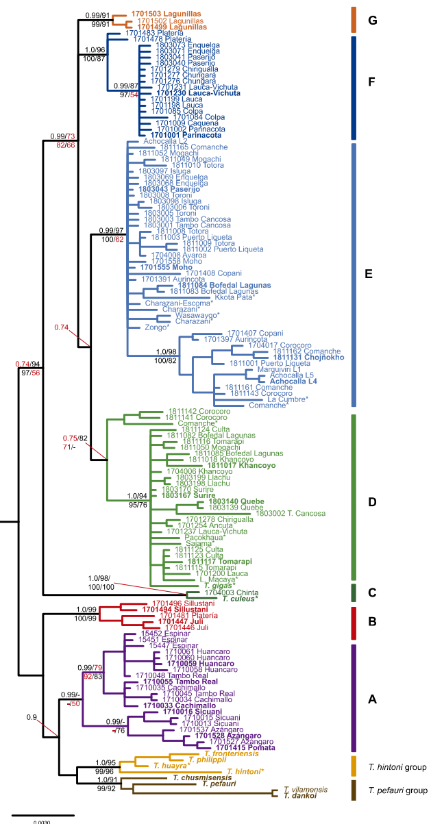
Fig. 2. Phylogenetic hypotheses for the Telmato-bius marmoratus complex obtained using Bayesian Inference (BI) with mitochondrial and nuclear genes combined. The numbers above and below the nodes correspond to the support values of posterior probabilities of BI, SH-aLRT and ultrafast bootstrap of Maximum Likelihood and Maximum Parsimony, respectively. Letters A to G correspond to the lineages recovered in this study. Low support values are shown in red. The outgroup was removed from the figure. * = samples only with mtDNA obtained from GenBank (see supplementary material S1). Tips in bold = samples used in species delimitation analyses. (For interpretation of the references to color in this figure legend, the reader is referred to the web version of this article.)
