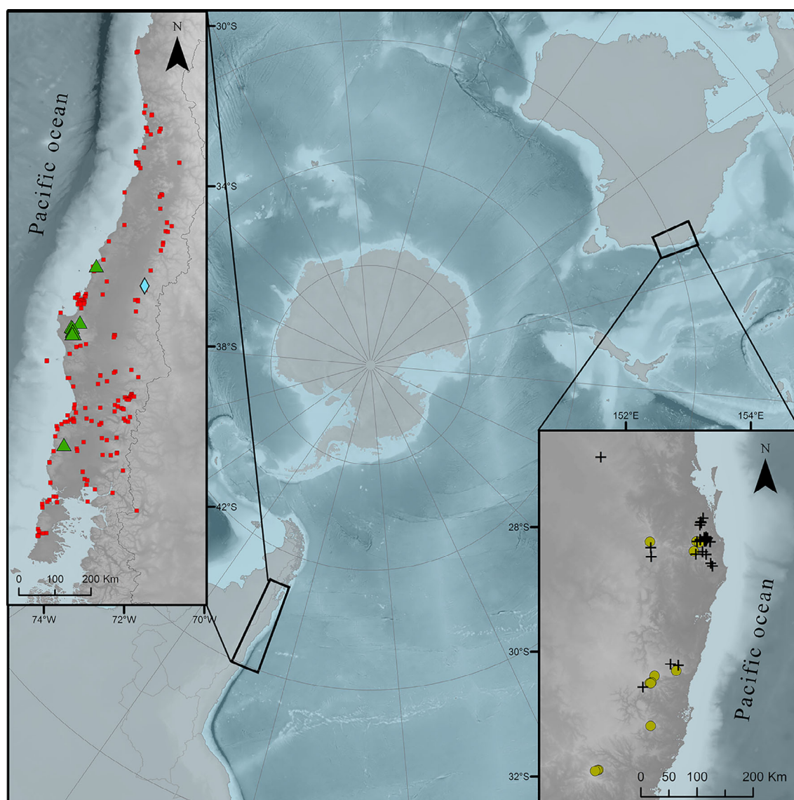
Fig. 1. Distribution map of Berberidopsidales: Streptothamnus moorei (black crosses), Berberidopsis beckleri (yellow circles), Aextoxicon punctatum (red squares), B. corallina (green triangles), and B. granitica (blue diamond).
