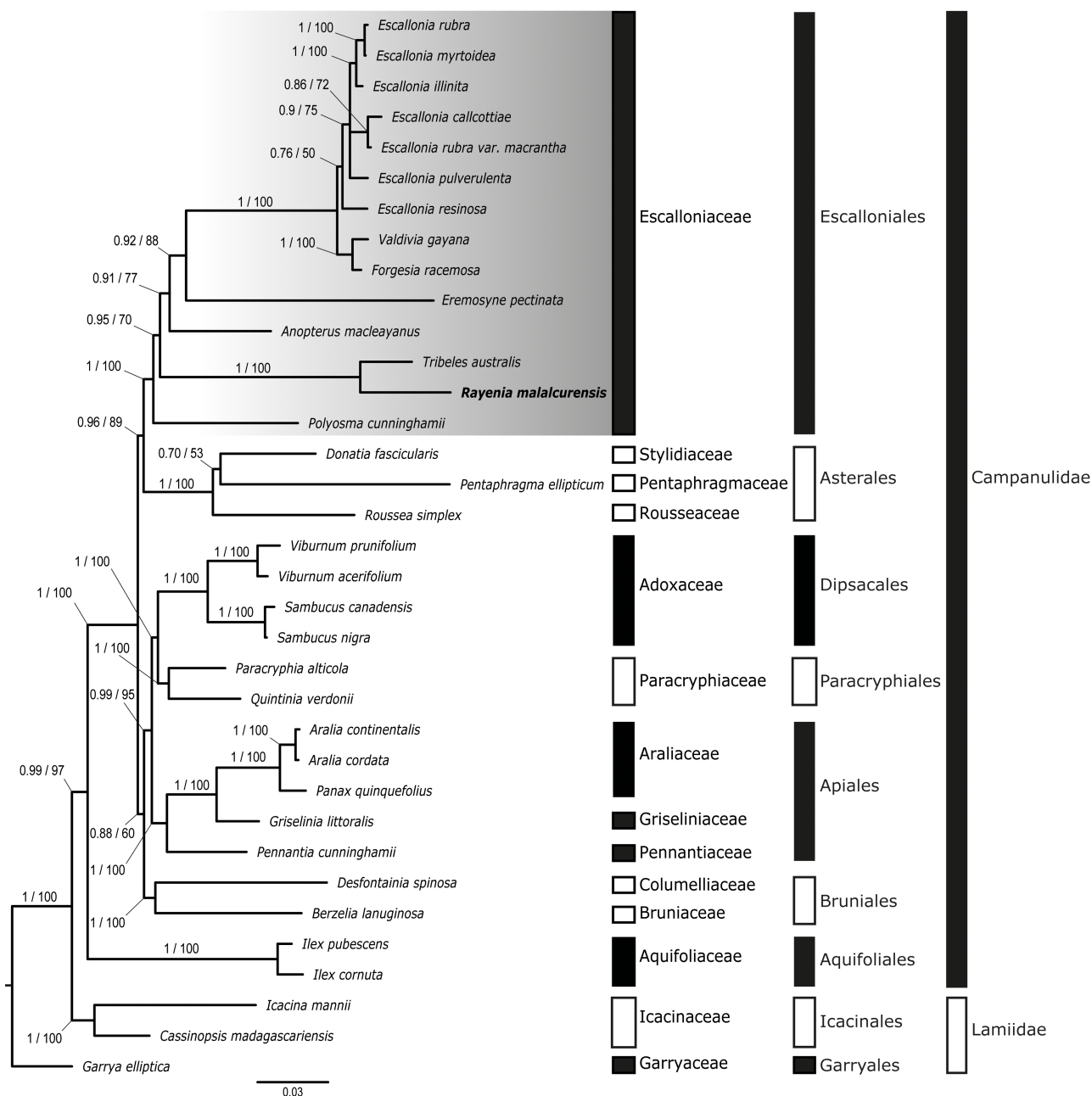
FIGURE 2. Phylogeny of Campanulidae resulting from Bayesian analysis of the combined plastid atpB , rbcL , matK , ndhF , rps16 , trnV-ndhC , trnS-trnG , trnL-trnF and PsbA-trnH dataset. Branch lengths indicate substitutions/site. Numbers next to the nodes represent the posterior probabilities from the BI analysis and bootstrap values from the ML analysis (PP/BS). The new proposed species, Rayenia malalcurensis is shown in bold.
