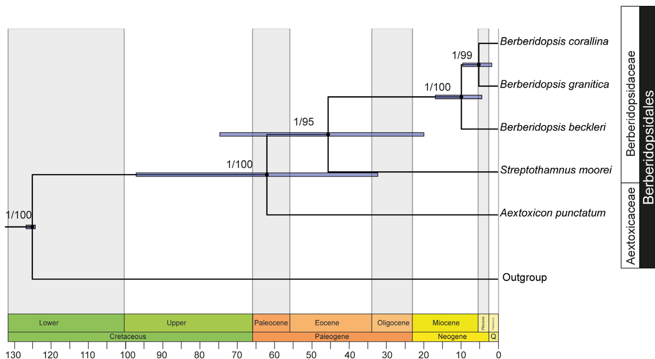
Fig. 2. Maximum clade credibility (MCC) tree of Berberidopsidales resulting from the Bayesian analysis of the combined nuclear and chloroplast dataset in BEAST. Numbers next to the nodes represent the posterior probabilities from the BI analysis and bootstrap values from the ML analysis (PP/BS). Blue bars represent 95% highest posterior density intervals for the node ages.
