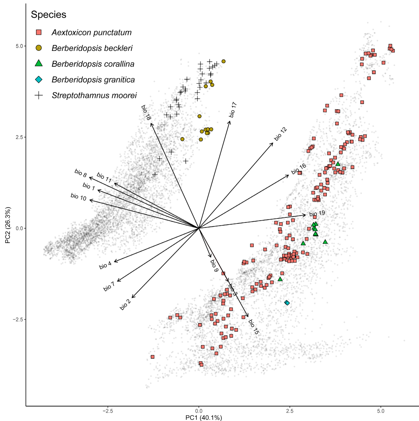
Fig. 3. Biplot of the two principal components extracted in the PCA of the 15 WorldClim v.2.1 bioclimatic variables (Fick & Hijmans, 2017). Light grey dots indicate environmental background values.
